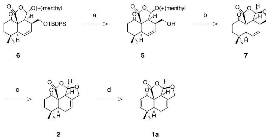
Scheme 3. a) TBAF, THF, room temp., 2 h; b) 20% TFA in CH 2 Cl 2 , room temp., 10 min, 92% over two steps; c) [(PPh 3 ) 2 Ir(CO)Cl] (50 mol %), toluene/ethanol (4:1, v/v), 70 °C, 6 h, 43% (ca. 35% of 7 was recovered); d) i. LDA, THF, -78 °C, 15 min, ii. PhSeBr, -78 °C, 15 min, iii. H 2 O 2 , 0 °C to room temp., 2 h, 58%.
