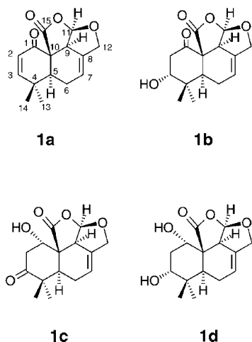
Figure 1. Anhydromarasmane 1a , marasmane 1b , isomarasmane 1c and dihydromarasmane 1d
